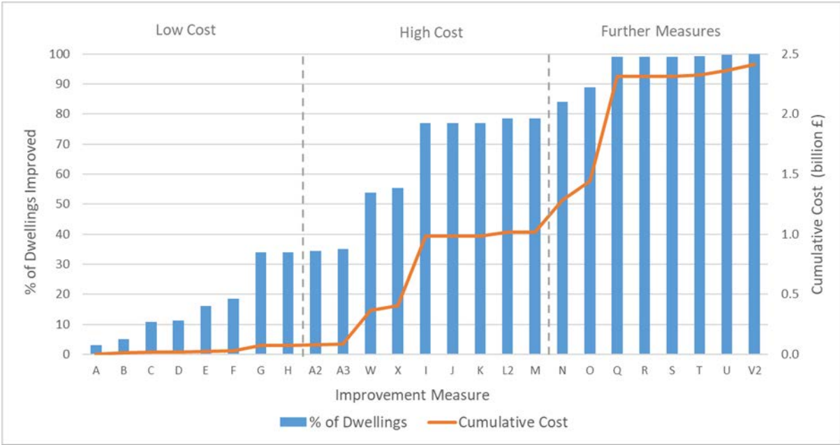
Figure 1: Percentage of dwellings improved to EER band C with each improvement, and the associated cumulative cost.
